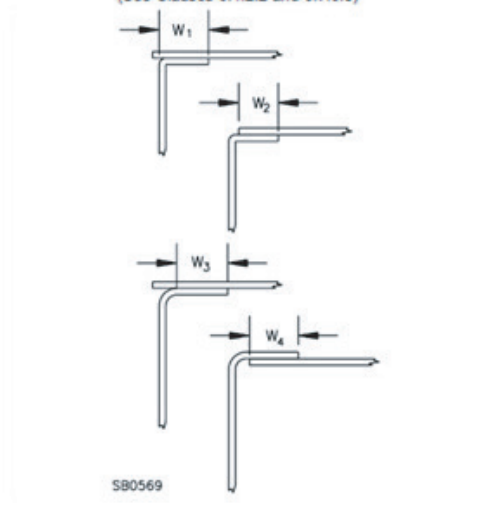
Figure 7 Overlap between flat cover and enclosure flange and at corner or enclosure seam (See Clauses 6.4.2.2 and 6.7.6.3)
