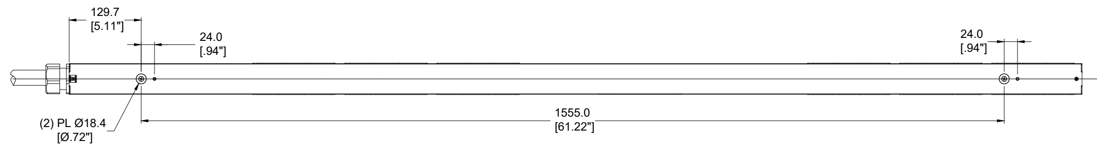
REAR VIEW
