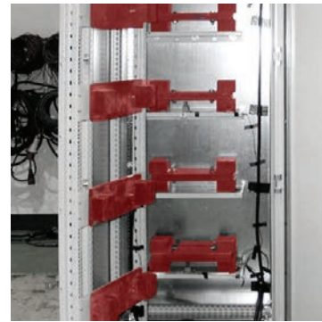
Figure 6. MCS20086R5 Loaded mounting plate and swing frame
