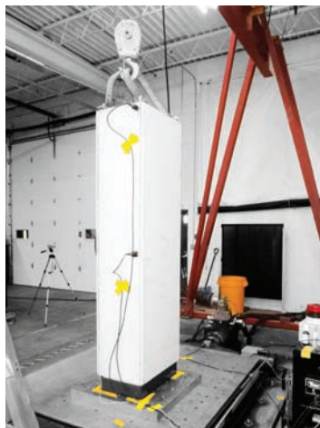
Figure 9. MCS20088R5 With seismic kit and seismic plinth
