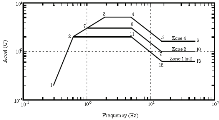
Figure 2. Required Response Spectra
