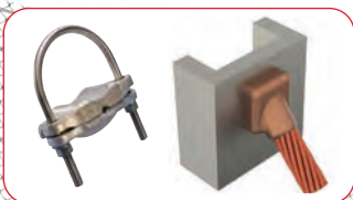
8. Fence bonding
