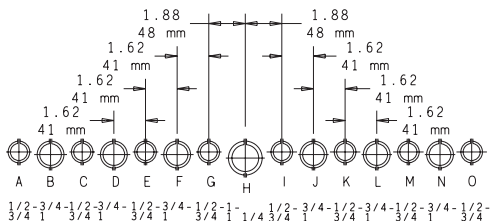
Conduit Sizes all Except ATC12R145 Knockout Pattern (From outside of box)
