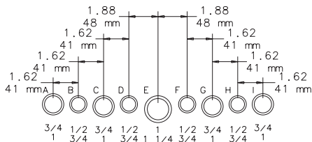
Knockout Pattern
