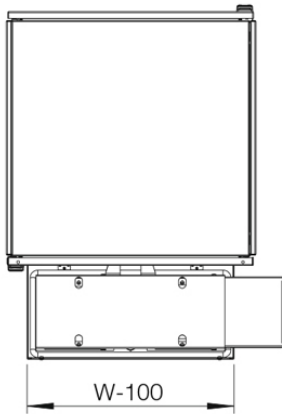
Sectional top view (without bottom plates)
