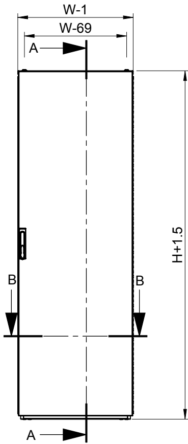
Front view
