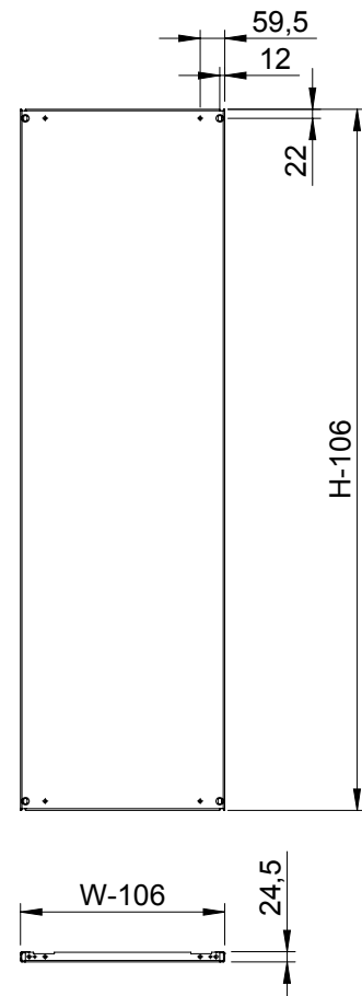
Mounting plate
