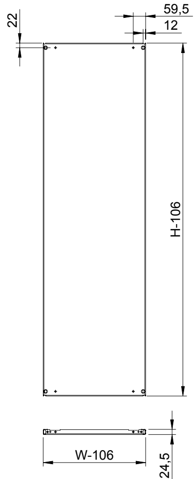
Mounting plate
