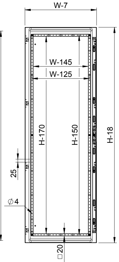
Mounting plate
