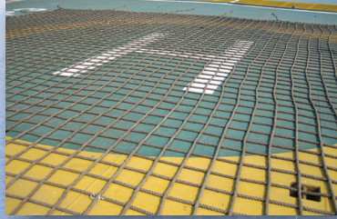
HELIDECK ■ Anti-icing
