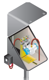
A pre-fabricated tubing bundle and enclosure can facilitate instrument winterization and reduce failure rate.
