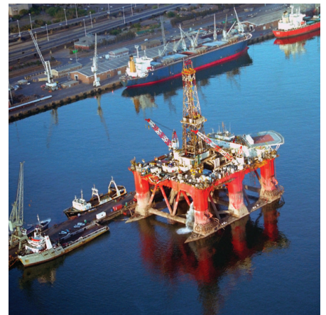
Semi-submersible Rig
