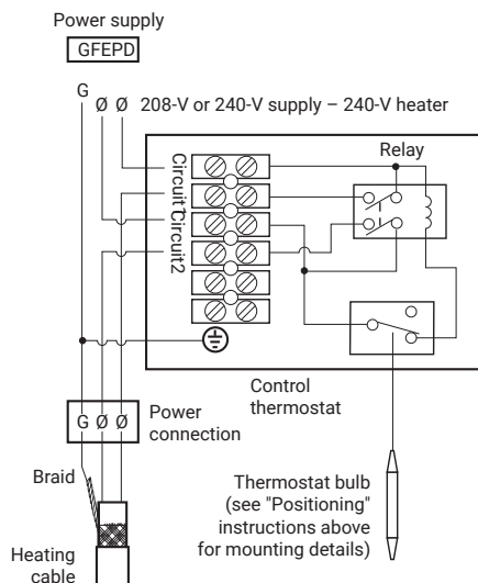
Figure 1. Heat-tracing control
