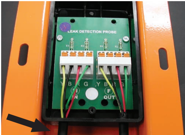
Figure 3. Multiple probe wiring configuration and suggested tie wrap location
