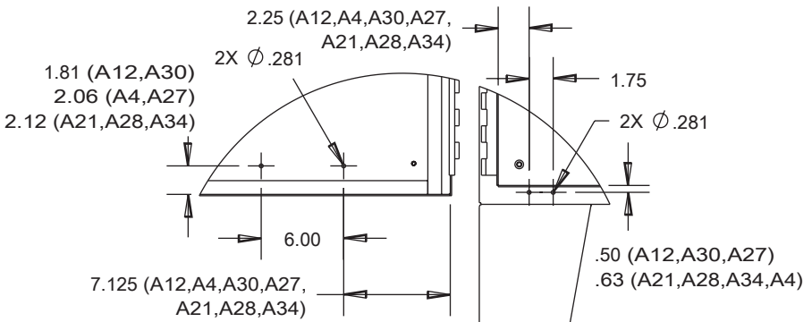
CONTINUOUS HINGE
