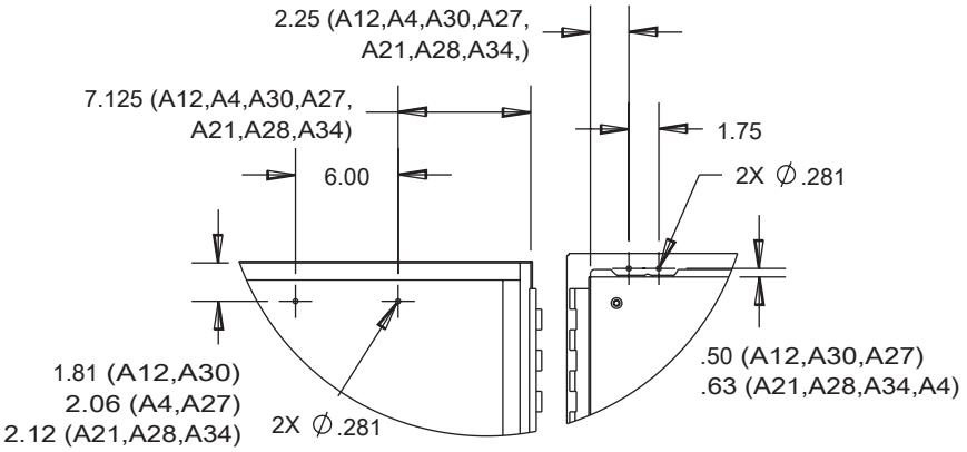
CONTINUOUS HINGE
