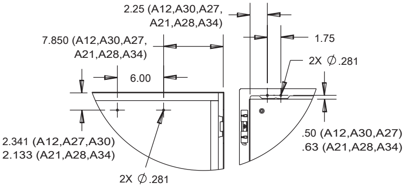
LIFT OFF HINGE
