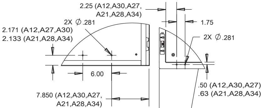
LIFT OFF HINGE
