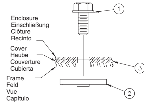
Frame Mounting Feld Montage Support D'Armature Montaje Del Marco
