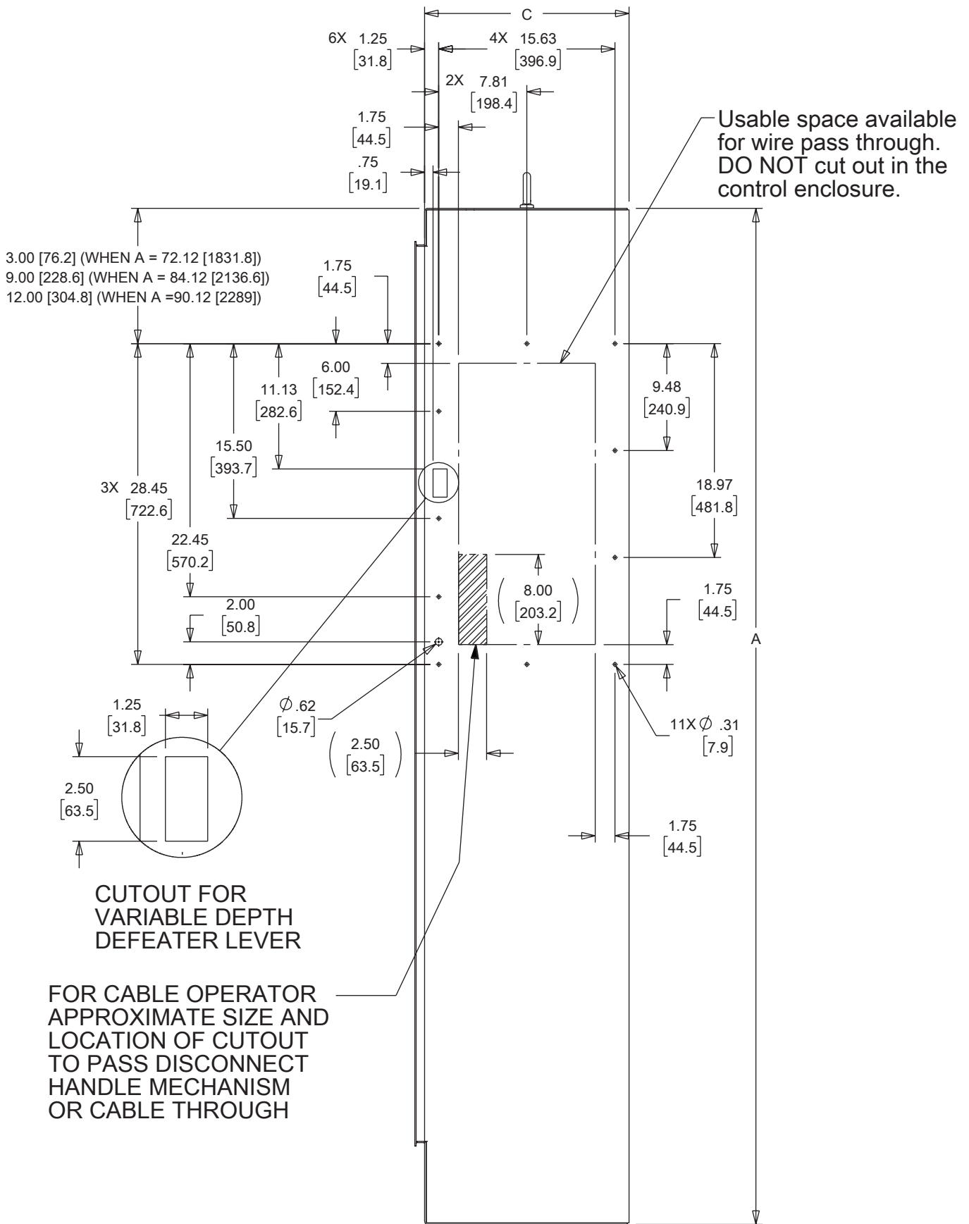
34 INCH SEQUESTR C = 18.12 [460.4] BUL - A28, A34, A4L3D, A28S4
