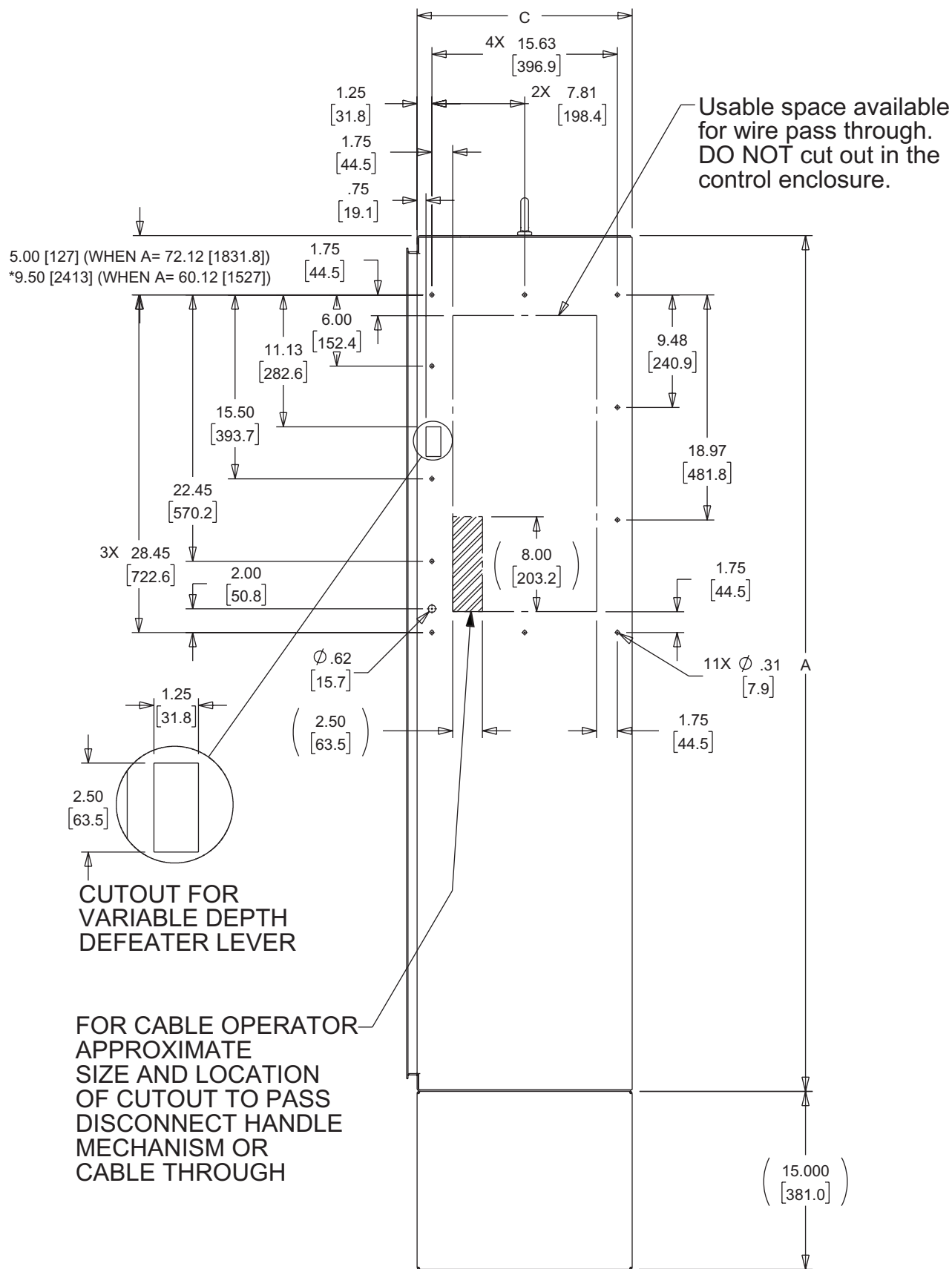
34 INCH SEQUESTR C = 18.12 [460.2] BUL- A21, A21S4
