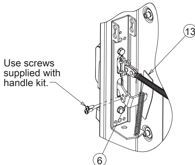
Square D Handle Figure 3A
