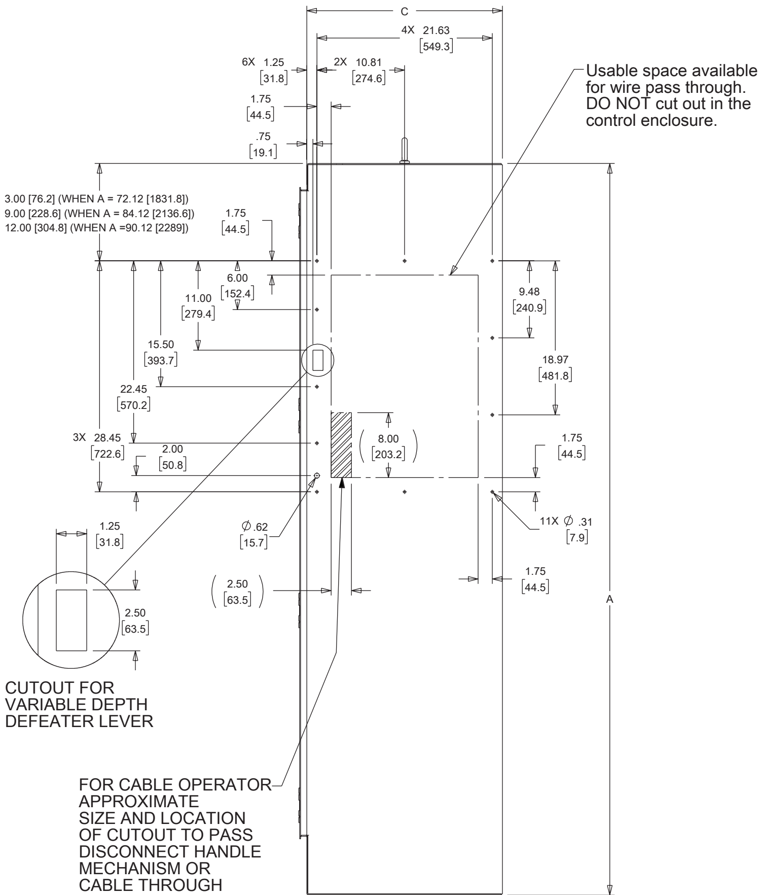
34 INCH SEQUESTR C = 24.12 [612.6] BUL - A28, A34, A4L3D, A28S4
