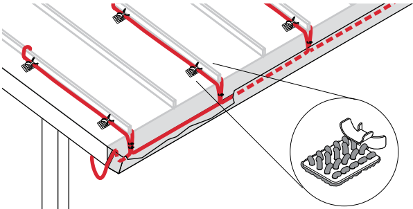
Figure 18: GMK-RC adhesive attachment
