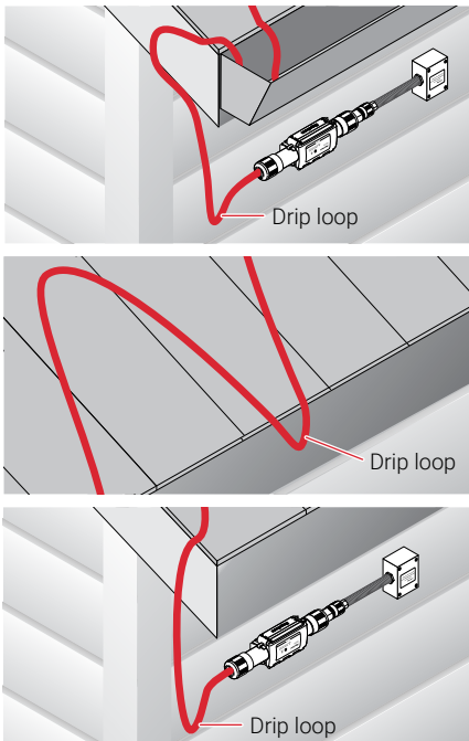
Figure 25: Drip loops
