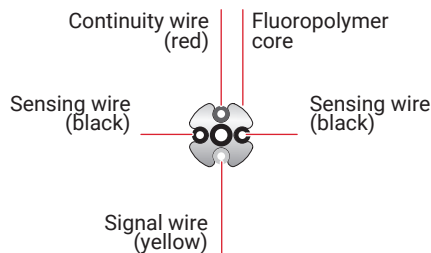
Cable construction
