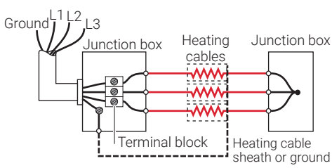
Figure 39: Typical 3Ø Wye connection
