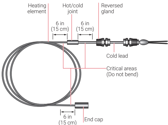
Figure 24: Typical tubular heater
