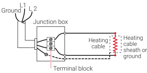
Figure 37: Typical 1Ø connection
