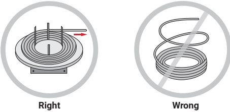
Figure 4: Unreeling/uncoiling cable
