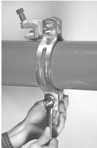
First tighten bolt that passes through brace clamp until the shear head on nut snaps off. Then proceed to tighten the other bolt on the CSBSTU until the shear head on nut snaps off.
