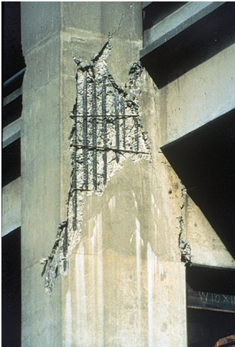
Lap splices transfer their load through the concrete and will fail as concrete cover degrades.
