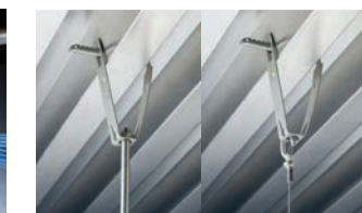
Threaded rod/chain/wire from trapezoidal steel decking
