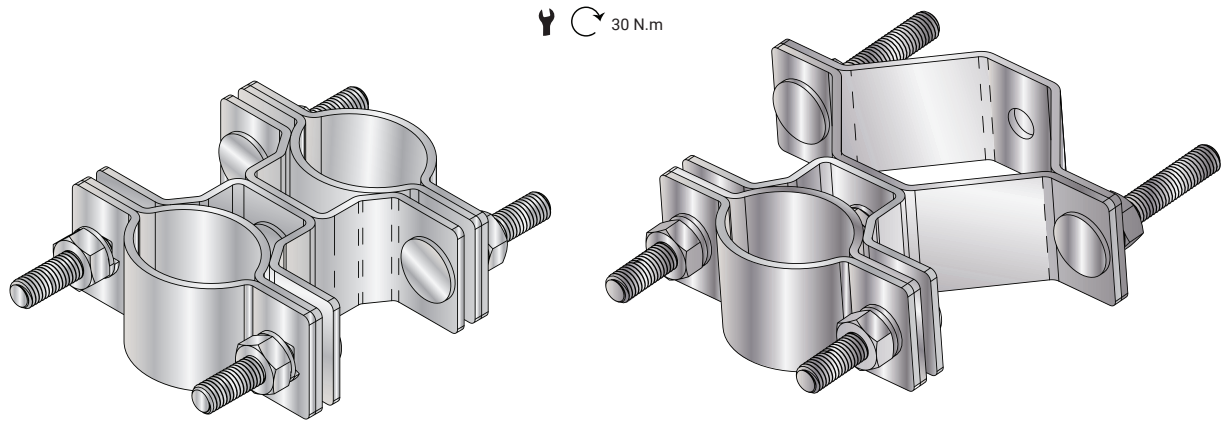
Figure 41 : Supports de mât ronds
