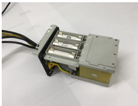
Step 4: The screw ejector lifts one end of the fuse, which may now be removed. Use of screw ejector mechanism avoids damaging the plastic tray.
