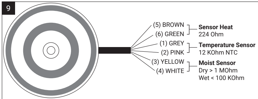
NTC 12 kΩ @ 25°C - RAYSTAT-M2-G-Sensor / RAYSTAT-M2-A-Sensor
