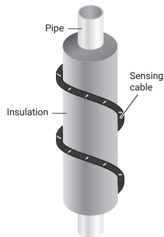
Vertical pipe
